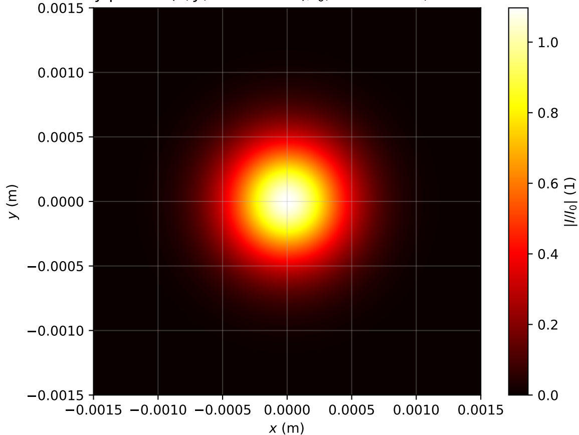
Intensity profile I(x, y, z = 0.398m)/I_0 , P_{in}=0.9P_{cr} , artificial time
